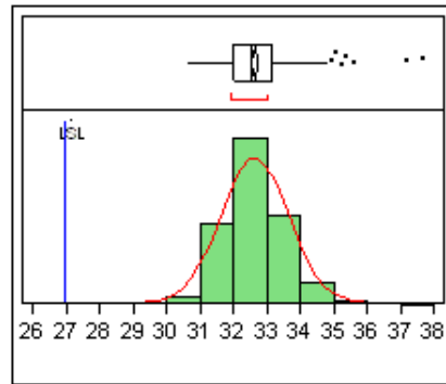
Figure 4. OIP3 Distribution@60mA.
