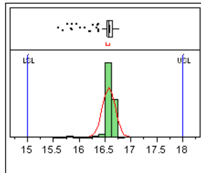
Figure 2. Gain Distribution@60mA.
